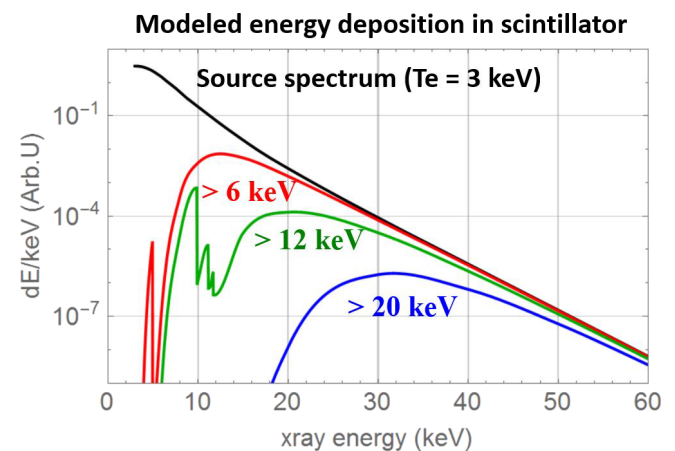
FIG. 5. PXTD response to x-rays from a T_e = 3 keV plasma. Ch1 is filtered with 181\text{-}\mu\text{m} Al+ 102\text{-}\mu\text{m} Ti. Ch2 is filtered with 181\text{-}\mu\text{m} Al+ 635\text{-}\mu\text{m} stainless steel. Ch3 is filtered with 181\text{-}\mu\text{m} Al+ 41\text{-}\mu\text{m} Ta. This calculation takes into account x-ray filter transmission, energy deposition in the scintillators, and light collection efficiency of the optics (e.g., effect of vignetting).
