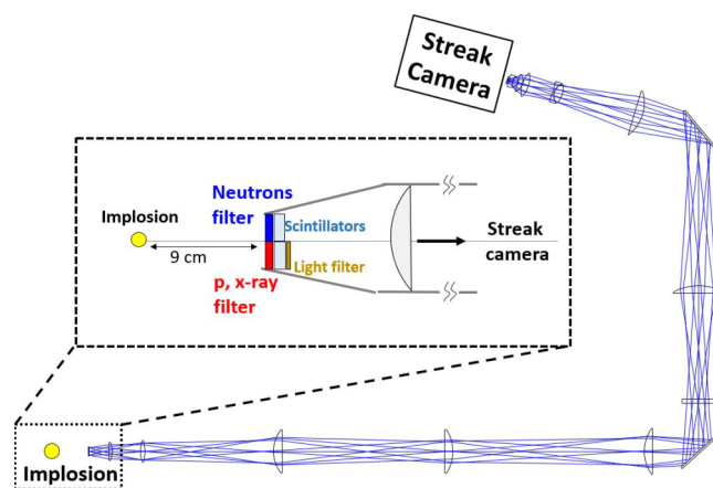
FIG. 1. Schematic of the PXTD design on OMEGA, which uses a 3.5-m optical relay to transport light from the scintillators positioned at 9 cm from the implosion to an optical streak camera outside the target chamber. The front end close to the implosion is visually expanded for clarity. Either a 2-channel or 3-channel scintillator setup is used in the nosecone. The 2-channel setup shown here houses two pieces of optically isolated scintillator, with filtering in front to measure neutrons, and proton/x-ray, respectively. A light attenuation filter is placed behind one of the scintillators to equalize the signals from the two channels.
