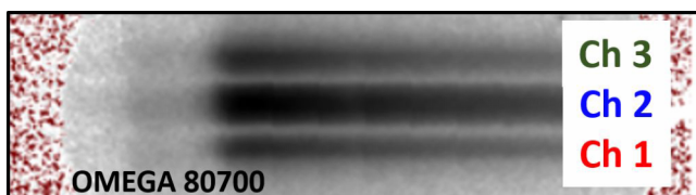
FIG. 4. PXTD x-ray flat-field streak image for OMEGA shot 80700. In this experiment, all three channels use the same x-ray and light attenuation filter. Vignetting of the optical system and differences in scintillator thickness contributed approximately equally to the spatial difference in the light distribution across the different channels (along the direction perpendicular to the streak).
