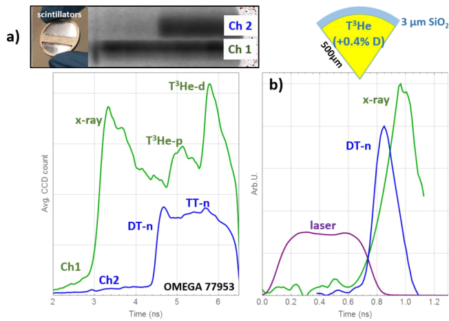
FIG. 8. (a) A proof-of-principle PXTD measurement of charged particles, neutrons, and x-ray signals from a T 3 He-gas-filled implosion (with 0.4% D contamination). (a) The top streak image illustrates the streak signals of x-rays, T 3 He-p, and T 3 He-d on channel 1, and the streak signals of DT-n and TT-n on channel 2. The bottom plot illustrates the lineouts (the streak image projected onto the time axis). (b) The DT-n reaction and x-ray (>12 keV) emission histories are relatively timed to each other to within \pm 10 ps, and absolutely timed to the laser drive. The 14.1-MeV DT-n and 9.5-MeV T 3 He-d are monoenergetic particles, whereas the T 3 He-p and the TT-n have broad, continuous energy spectrum. Ch1 is filtered with 40- \mu m Ta+40- \mu m Al, and Ch2 is filtered with 540- \mu m Ta+40- \mu m Al.
