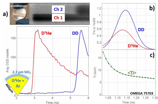
FIG. 6. Simultaneous PXTD measurements of the 14.7-MeV D^3\text{He} -p and the 2.45-MeV DD-n burn histories from a thin-glass, D^3\text{He} -gas-fill implosion on OMEGA shot 75703. (a) The streak image illustrates the streak of the DD-n signal (top part of image) and the D^3\text{He} -p signal (bottom-part of image). The bottom part of (a) illustrates the 14.7-MeV D^3\text{He} -p and 2.45-MeV DD-n streak lineouts (the streak image projected onto the time axis). At 9 cm away from the implosion, the D^3\text{He} -p arrives about 2.5 ns before the DD-n. (b) D^3\text{He} -p and DD-n burn histories determined from the data in (a) using a forward-fitting method which includes a model of the PXTD response. (c) Time-resolved ion temperature T_i(t) inferred from the ratio of the DD and D^3\text{He} nuclear reaction rates shown in (b). See text for more details.
