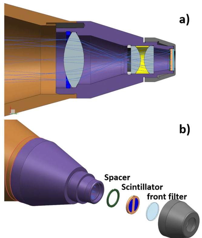
FIG. 10. (a) Sliced view of the new 3-cm PXTD nosecone design. Three new lenses are added in the new (purple) nosecone to relay light from the new scintillator plane at 3 cm. (b) Exploded view of the new 3-cm PXTD nosecone design.
