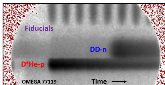
FIG. 2. PXTD streak image from a D^3He -gas-filled implosion (OMEGA 77119). The streak signal is produced by the 14.7-MeV D^3He -p and 2.45-MeV DD-n from the implosion. The OMEGA fiducials, spaced 548 ps apart, appear at the top of the streak image and are used for absolute timing relative to the laser pulse.
