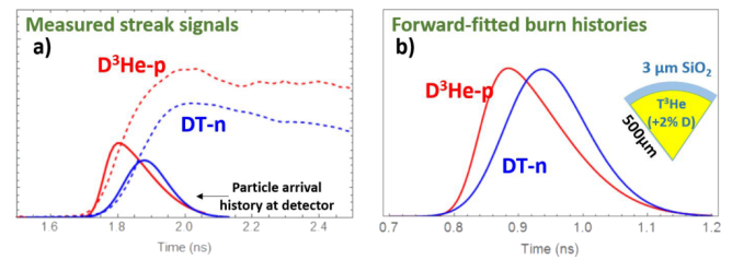
FIG. 9. (a) Measured D 3 He- and DT streak lineouts (dashed) and deconvolved signals (solid) representing the particle arrival histories at the PXTD scintillator. In this case, the DT-n and D 3 He-p burn histories are simultaneously determined with a relative precision of \sim 10 ps for this thin-glass shock-driven implosion with T 2 + 3 He fill, with a trace amount of D 2 . The forward-fitted D 3 He-p and DT-n burn histories shown in (b), normalized to illustrated differences in shape.
