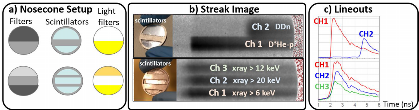
FIG. 3. (a) PXTD scintillator(s), x-ray filter, and light attenuation filter configurations for the different measurements. (b) Measured D^3He -p and DD-n streaks simultaneously using two channels (top row), and three measured x-ray streaks at different energy bands using three channels (bottom row). As indicated by (a), each streak channel has its own filtering in front of, and light attenuation filter behind, the scintillator to equalize the signal relative to the other channels. (c) Projected nuclear-reaction and x-ray lineouts. The filtering for the multiple nuclear reactions (top row) and x-ray emission (bottom row) cases will be discussed in details in Secs. III A and III B, respectively.
