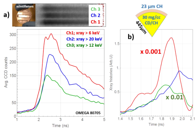
FIG. 7. Simultaneous PXTD measurements of emission histories of x-rays with energies above 6 keV, 12 keV, and 20 keV from a thick-CH implosion on OMEGA. (a) The top image illustrates the streak of the three x-ray signals, while the bottom plot illustrates the x-ray lineouts (the streak image projected onto the time axis). (b) Deconvolved x-ray emission histories determined from the lineouts shown in (a). These emission histories were determined by considering and correcting for the PXTD response, light filter transmission, and channel efficiency. The filtering for these three channels is described in Figure 5. In (b), channel 1 (red) and channel 3 (green) are scaled by 0.001 and 0.01, respectively, to display all three signals on the same scale.
